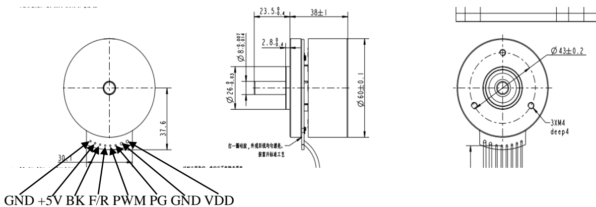
FIG. 1 Mechanical dimensions
